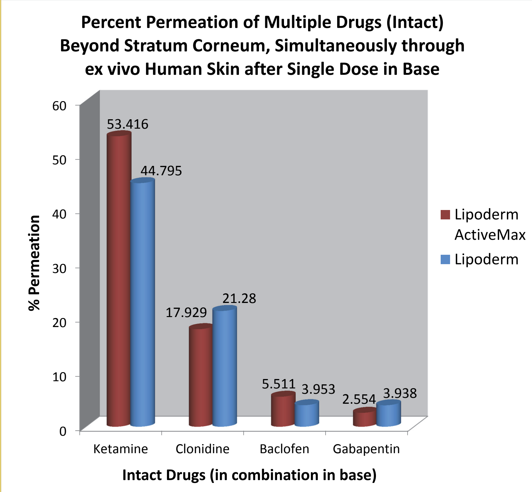
Figure 2. Percent permeation of the four active substances
