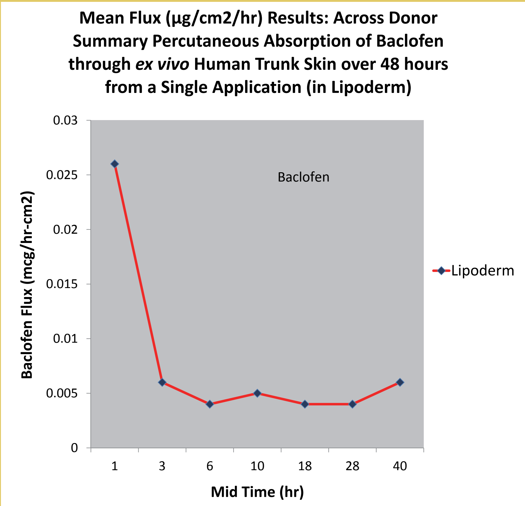
Figure 4. Baclofen flux versus time
